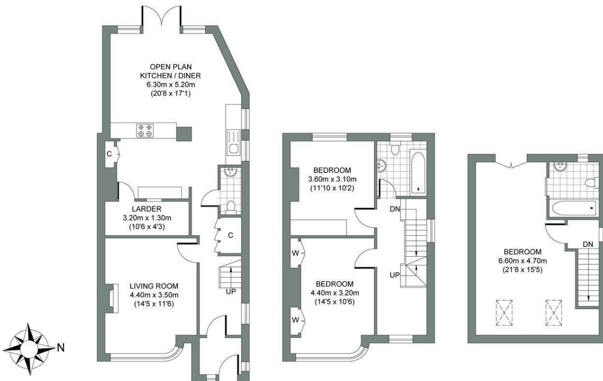
GROUND FLOOR Approximate Gross Internal Area 61.94 sq m / 666.71 sq ft
